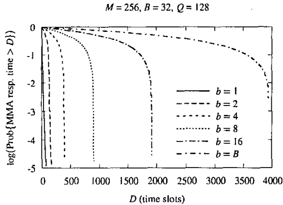
Fig. 4. Complementary distribution function of the MMA response time for Q = 128 and different values of b .
