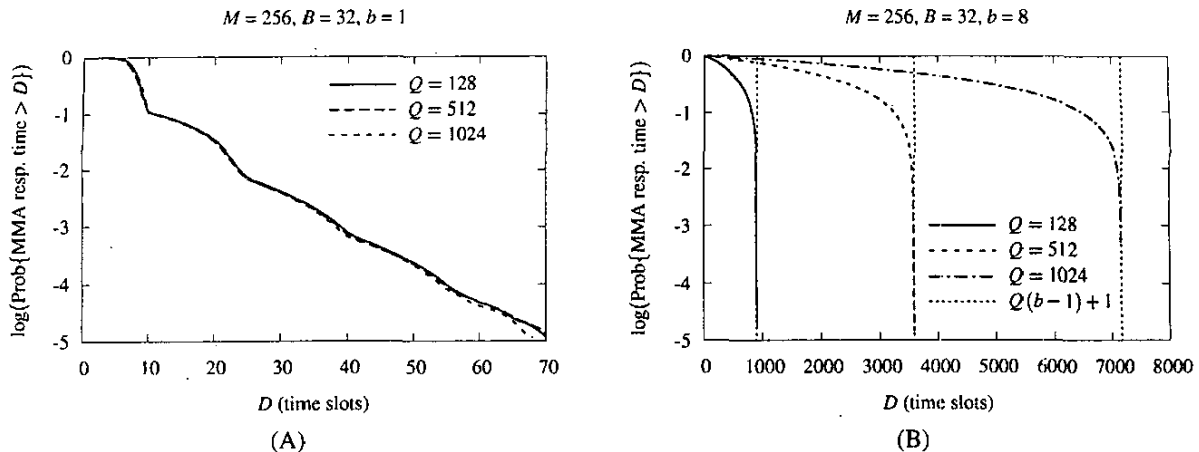
Fig. 3. Complementary distribution function of the MMA response time for different values of Q and b = 1 (A), and b = 8 (B).
